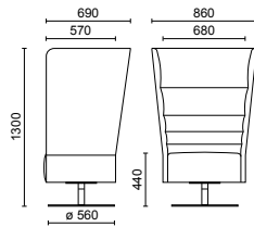
1 SWIVEL SEATER WITH CENTRAL ROUND STEEL BASE
