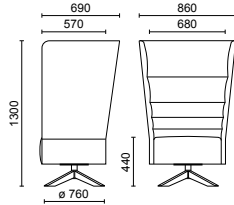
SINGLE-SEATER, SWIVELLING, 4-STAR BASE IN WOOD
