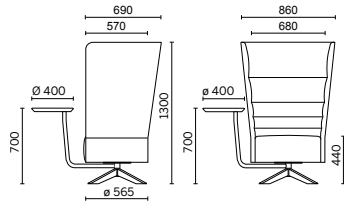
SINGLE-SEATER, SWIVELLING, 4-STAR BASE IN WOOD, SWIVELLING TABLET WITH SWIVELLING SUPPORT
