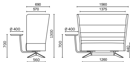
2-SEATER, 4-STAR BASE IN WOOD, SWIVELLING TABLET WITH SWIVELLING SUPPORT
