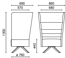
SINGLE-SEATER, BASE WITH 4 LEGS IN WOOD
