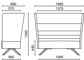
2-SEATER, BASE WITH 4-LEG IN WOOD
